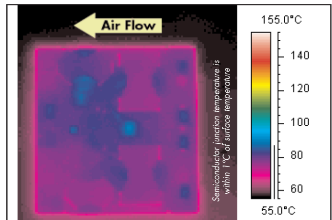
Figure 6: Thermal plot of converter at 20 amp load current with 55°C air flowing at the rate of 200 LFM. Air is flowing across the converter from output to input (nominal input voltage).
